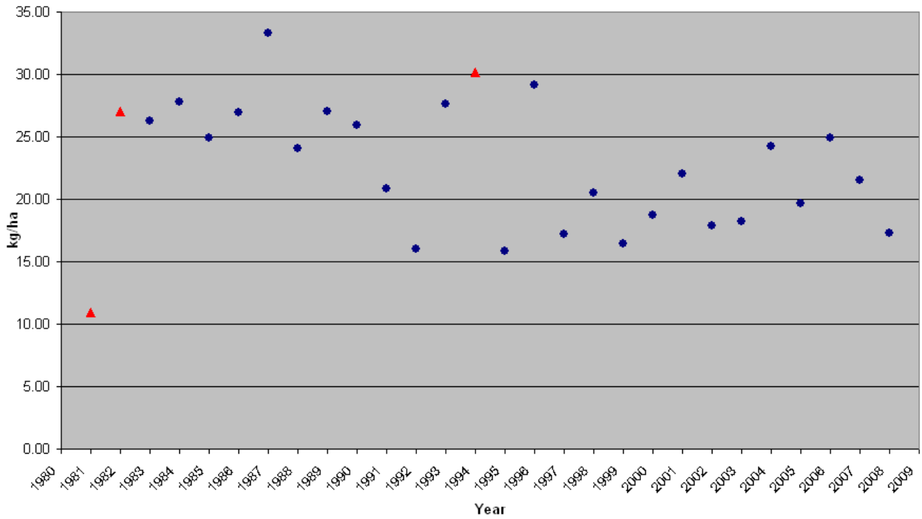
Figure 3 Sulfate (SO 4 ) NADP/NTN Site NJ99 (Washington Crossing State Park) Annual Wet Depositions (1981 - 2008) Kilograms Per Hectare (kg/ha)
