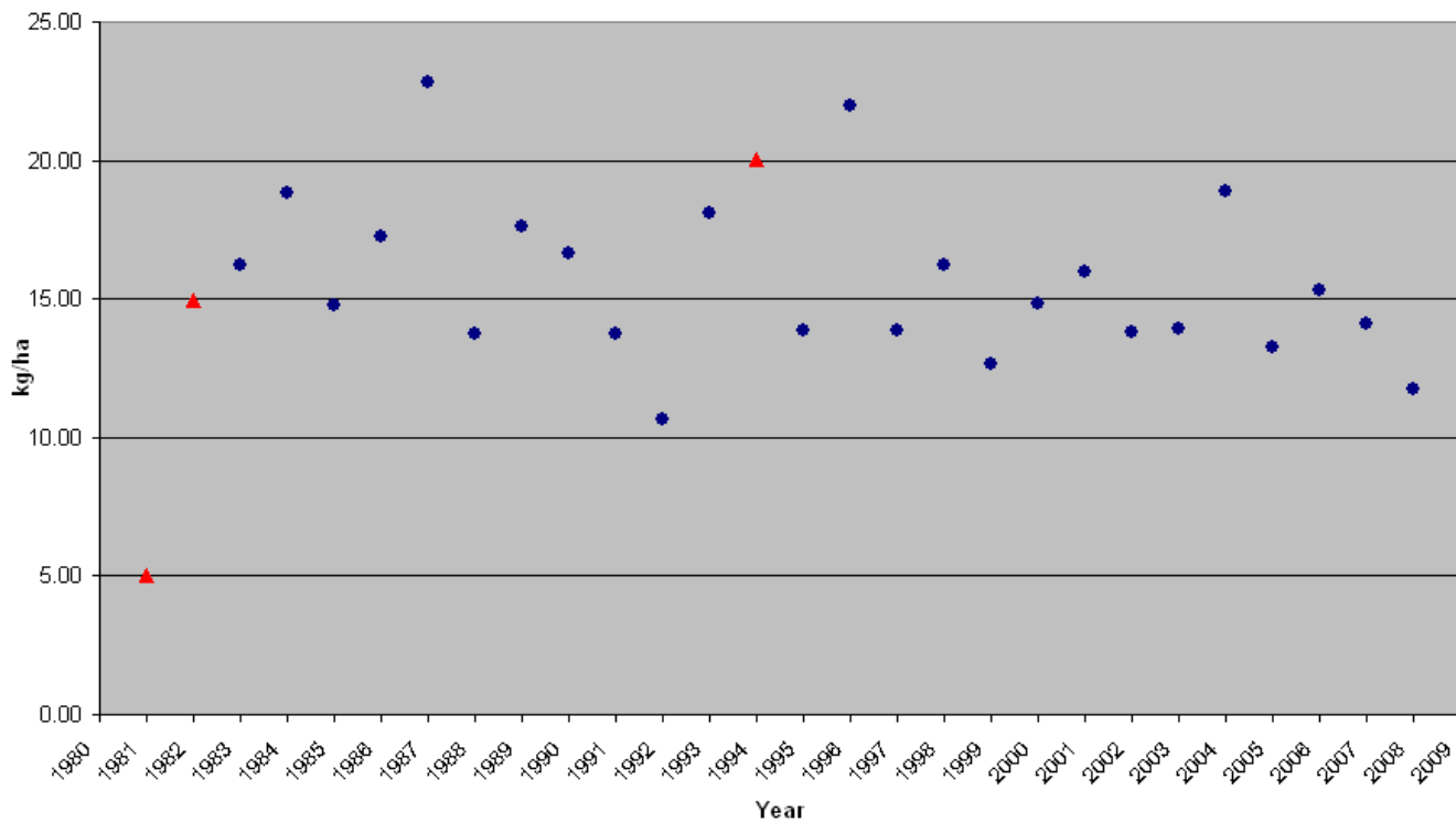
Figure 5 Nitrate (NO 3 ) NADP/NTN Site NJ99 (Washington Crossing State Park) Annual Wet Depositions (1981 - 2008) Kilograms Per Hectare (kg/ha)
